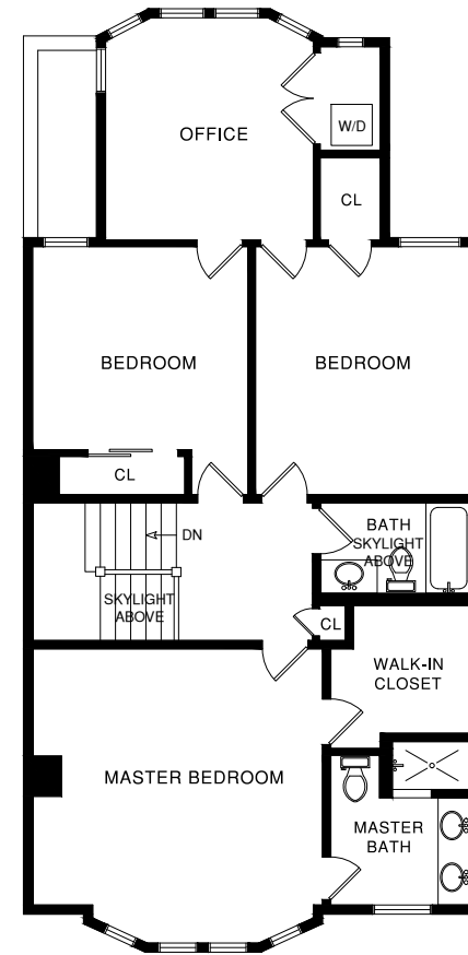
UPPER LEVEL
